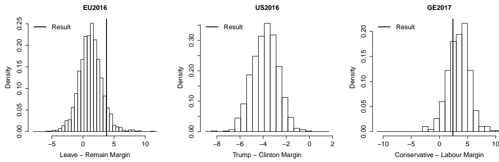
Figure 1: Posterior predictive distributions and results for national vote share margin, in the referendum (left), the presidential election (center), and in the general election (right).
